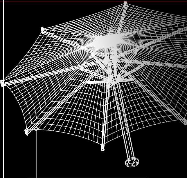
8-Point Twillite Wire Frame Model
