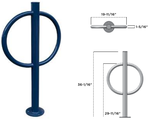
5040SM Hlare Rack, ultra blue
