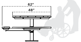
338H3 (Single-Sided Accessibility)
